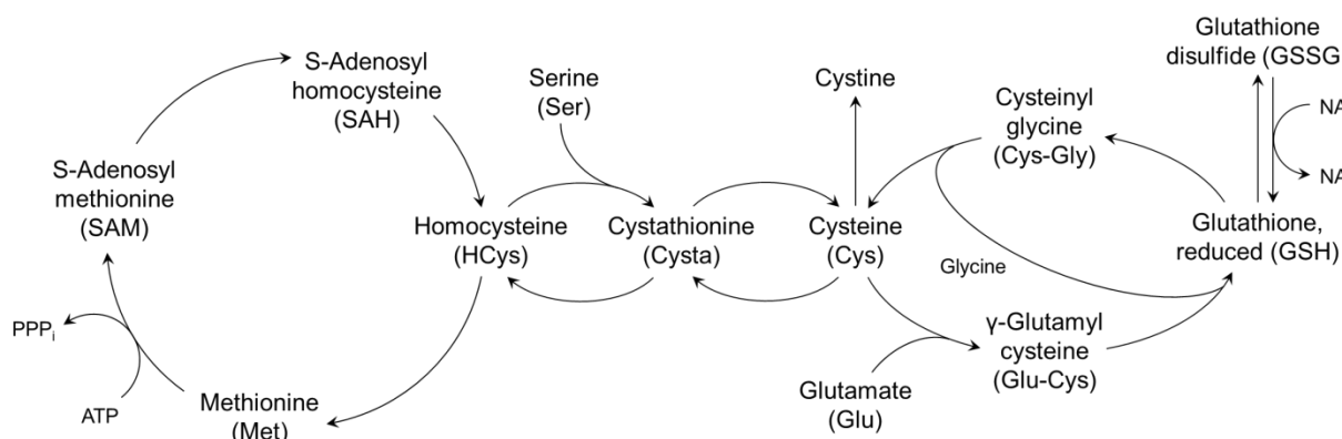
Figure 1. Reactions of the sulfur metabolic pathway intermediates 13,22 .
