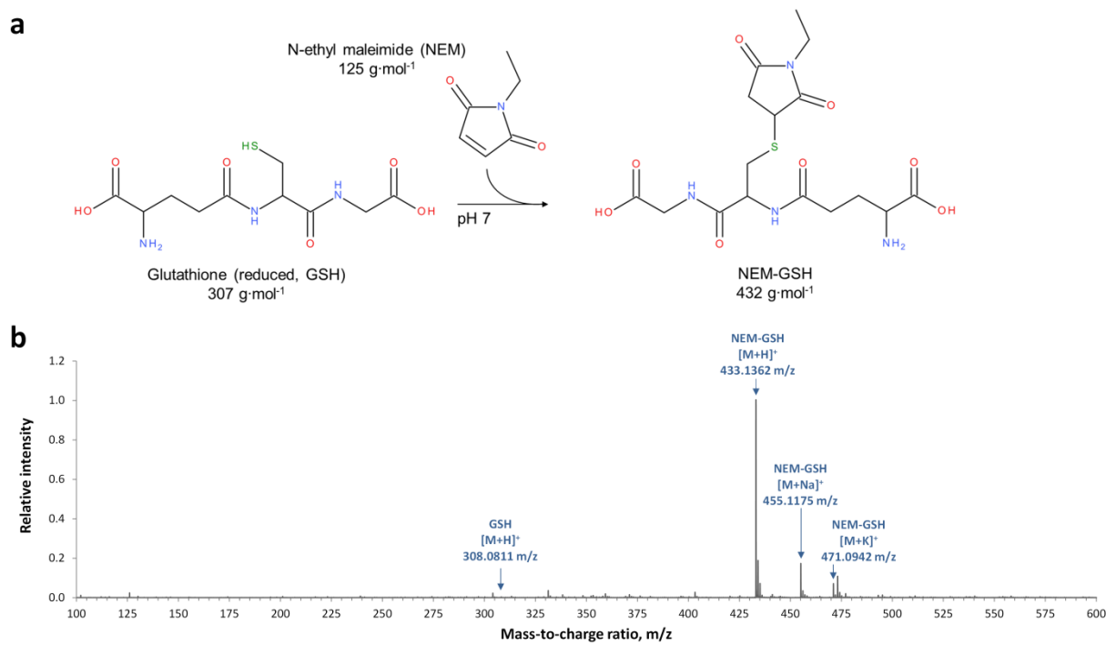
Figure 2. Thiol group derivatization with N-ethyl maleimide on the example of the formation of NEM-GSH from reduced glutathione. a) The double bond of the maleimide reagent forms a stable thioether bond with the sulfhydryl group at pH 7. b) Flow injection-TOFMS analysis of a single standard of glutathione after incubation with a 10-fold excess of NEM for 15 min at room temperature.
