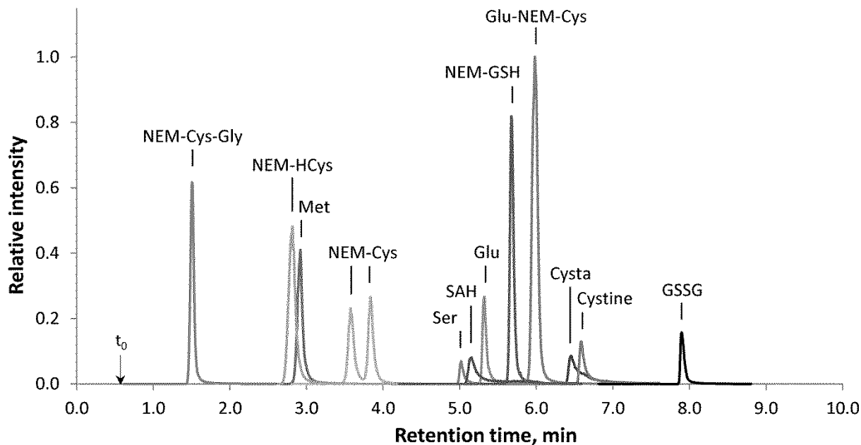
Figure 3. Representative chromatogram from HILIC-ESI-MS/MS analysis of sulfur metabolic pathway intermediates. The sample was prepared from metabolite standards in 90% acetonitrile (1 \mu M each, except for cystine and GSSG – 5 \mu M). Data were acquired on a Thermo TSQ Vantage triple quadrupole MS/MS system in SRM mode (Table 1).
